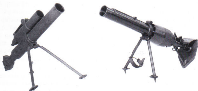
Although most Polish weapons were foreign types manufactured under licence, there were some local designs. Three wz. 36 45mm infantry mortars were deployed in each infantry company. The example on the left without the baseplate is the standard wz. 36, while the example to the right is the original version tested in 1932-33. (Ordnance Museum, APG)
