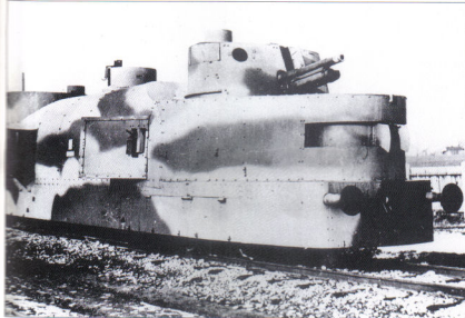
Armoured Train No.53 Smialy supported Army Lodz in the border battles and took part in the fighting with 4th Panzer Division near Mokra on 1 September. It had two armoured gun carriages like this one, each with two turreted wz. 02/26 75mm guns. These guns were effective against the thinly armoured German tanks, but the trains were vulnerable to Stuka attack. (J. Magnuski)
